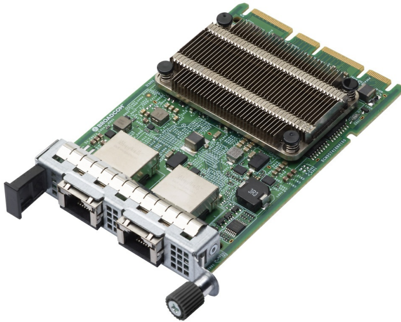
Figure 3. ThinkSystem Broadcom 57416 10GBASE-T 2-port OCP Ethernet Adapter
